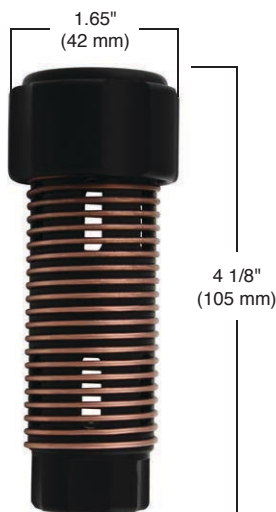
Figure 10-17 Biofoul Screen Dimensions
